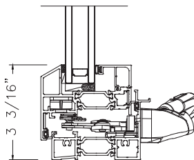
2C SILL AWNING ROTO OPERATOR INSULATED
