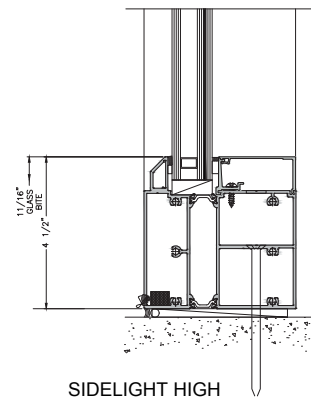
SIDELIGHT HIGH
