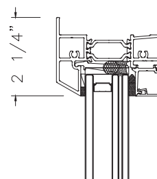
1C HEAD FIXED FLANGE
