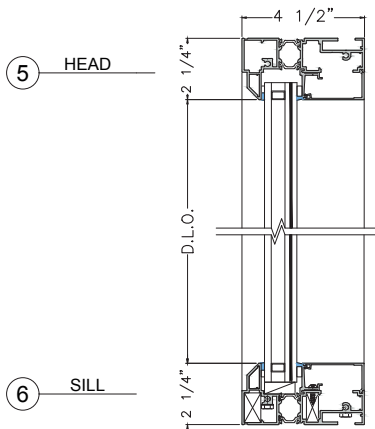
SIDELIGHT SILL
