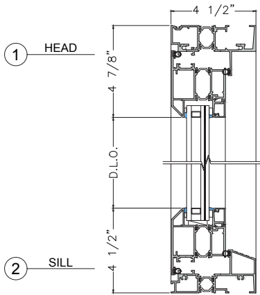
STANDARD SILL
