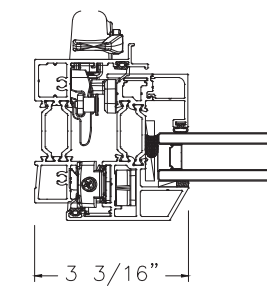
3C JAMB AWNING ROTO OPERATOR INSULATED
