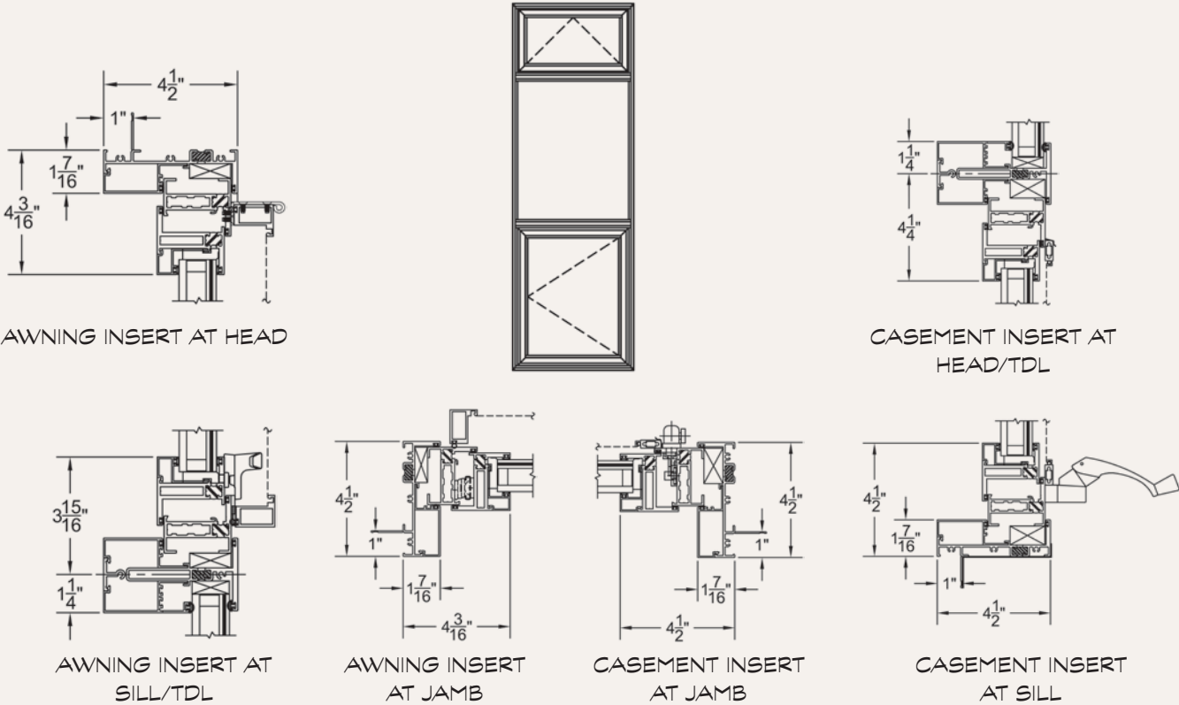
ELEVATION VIEW: O/O/O-GTF w/Awning and Casement Inserts
