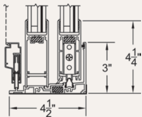
HIGH WATER SILL
