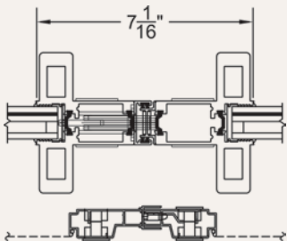
HP2-T MEETING STILES
