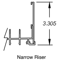
Narrow Riser
